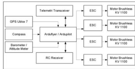
Fig. 4. Basic Quad Rotor Electronic Configuration System
