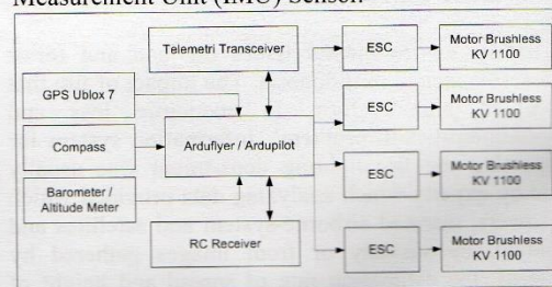
Fig. 4. Basic Quad Rotor Electronic Configuration System
