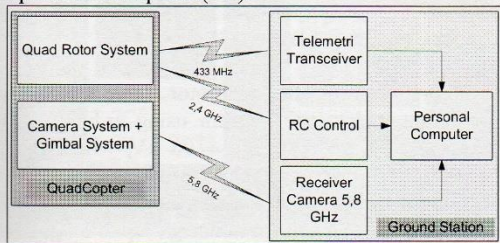
Fig. 6. Proposed Quad Rotor Configuration System
