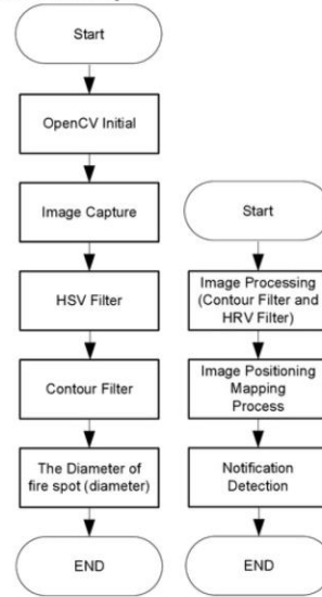
Fig. 8. Proposed fire monitoring flow chart
