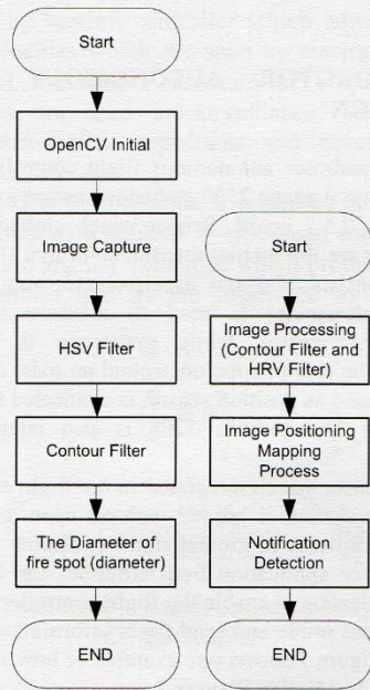
Fig. 8. Proposed fire monitoring flow chart
