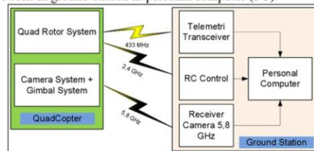
Fig. 6. Proposed Quad Rotor Configuration System
